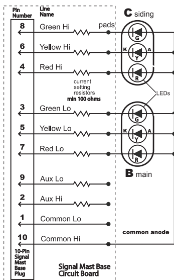
Wiring For B (main) and C (siding)
