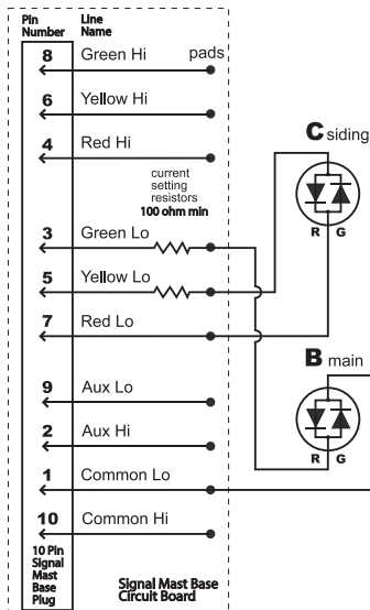
Wiring For B (main) and C (siding)
