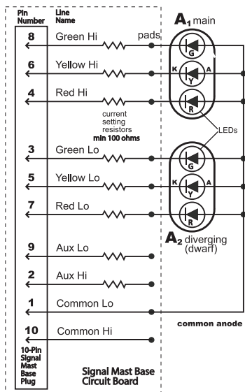
Wiring for A 1 (main) and A 2 (diverging-dwarf)
