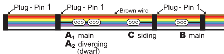
Signal Driver Cable Example
