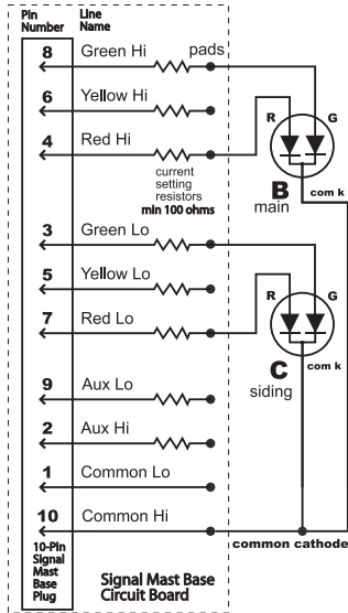
Wiring For B (main) and C (siding)
