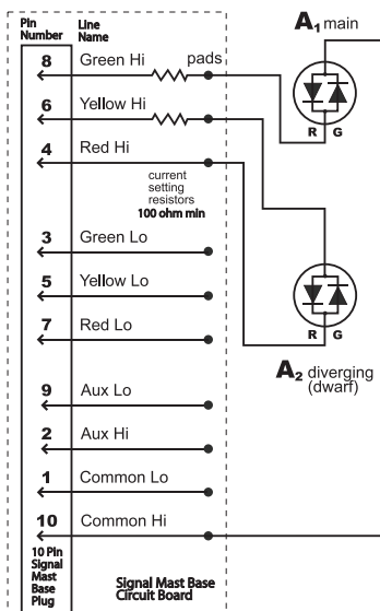
Wiring for A 1 (main) and A 2 (diverging or dwarf)
