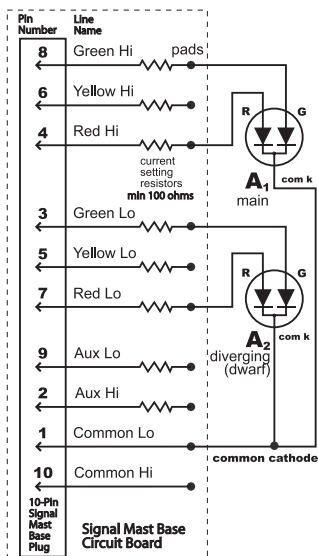
Wiring for A 1 (main) and A 2 (diverging or dwarf)
