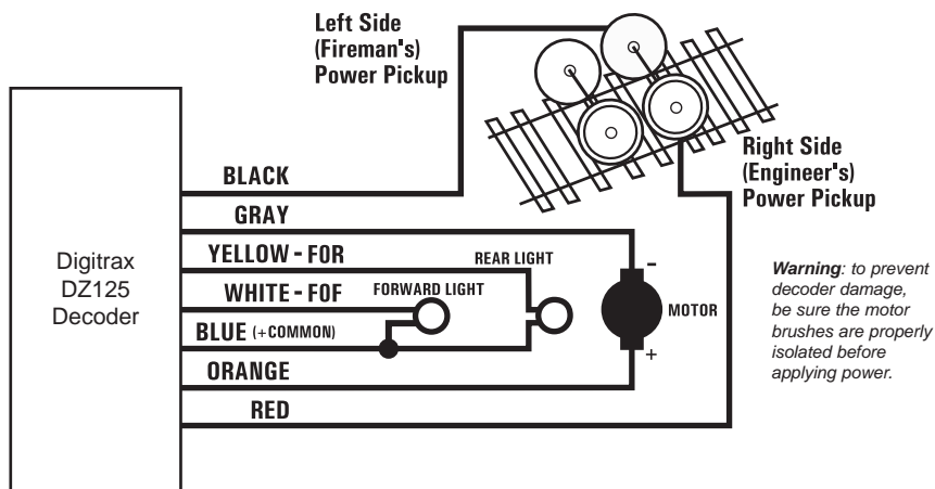
Figure 1. DZ125 Wiring Diagram
